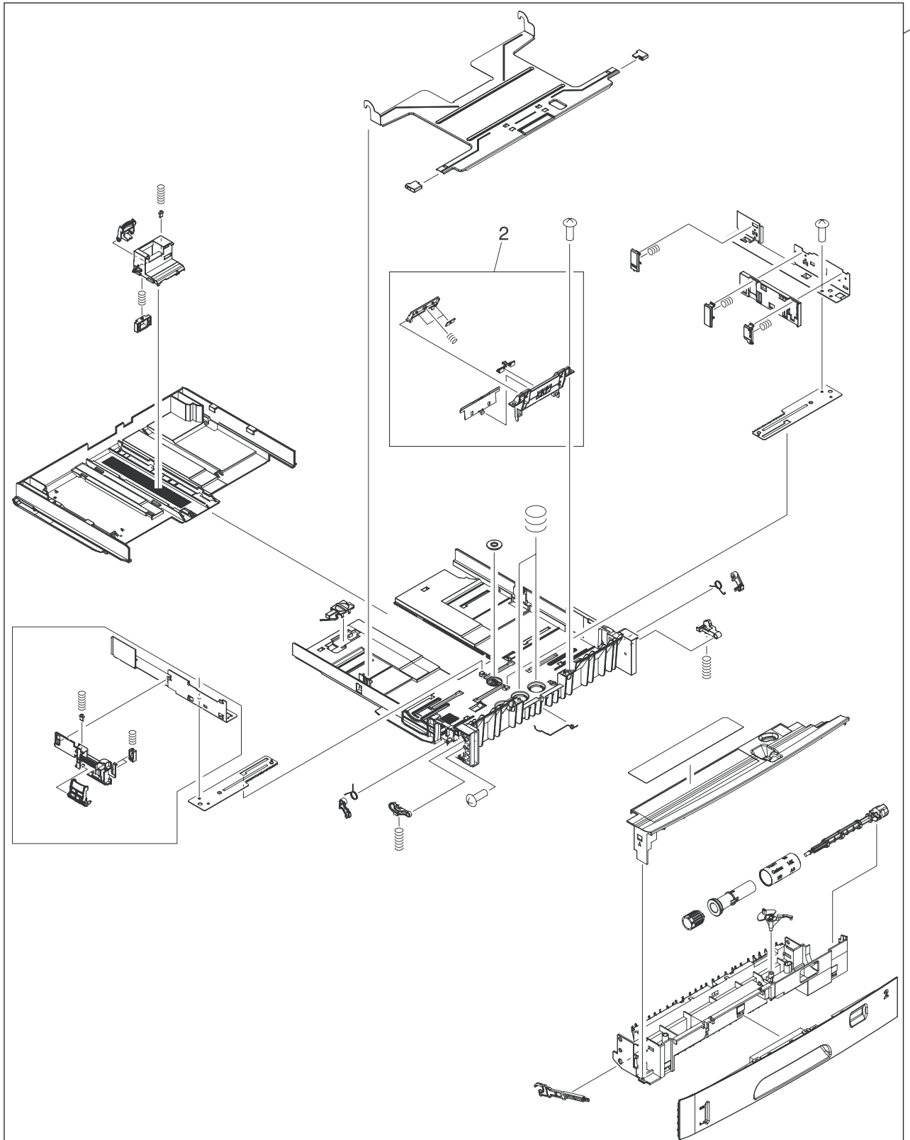
Figure 7-11 Cassette (tray 2)
