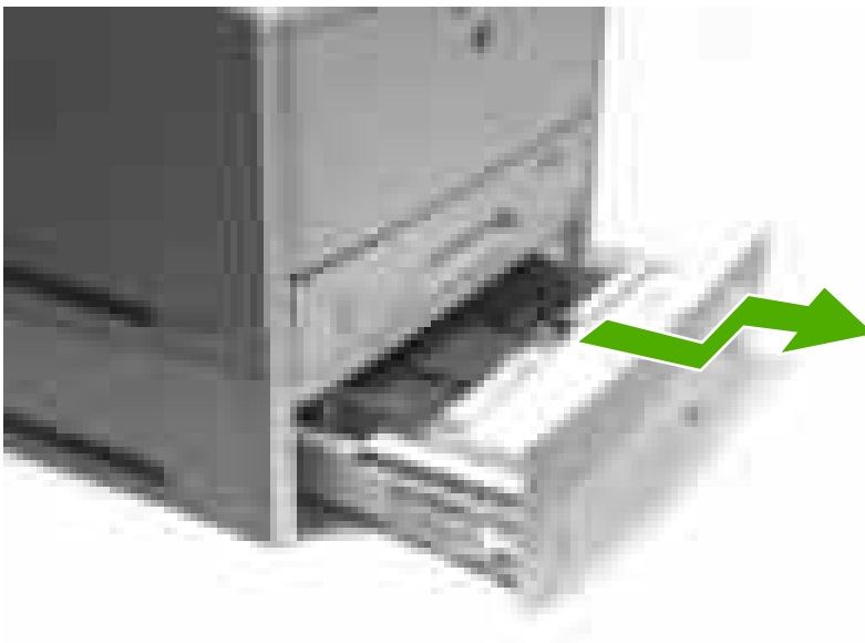
Figure 5-11 Removing the tray 3 retard roller (1 of 2)
