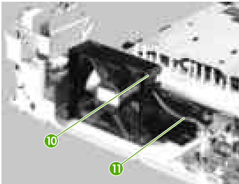
Figure 5-174 Removing the duplexer fan (5 of 5)
