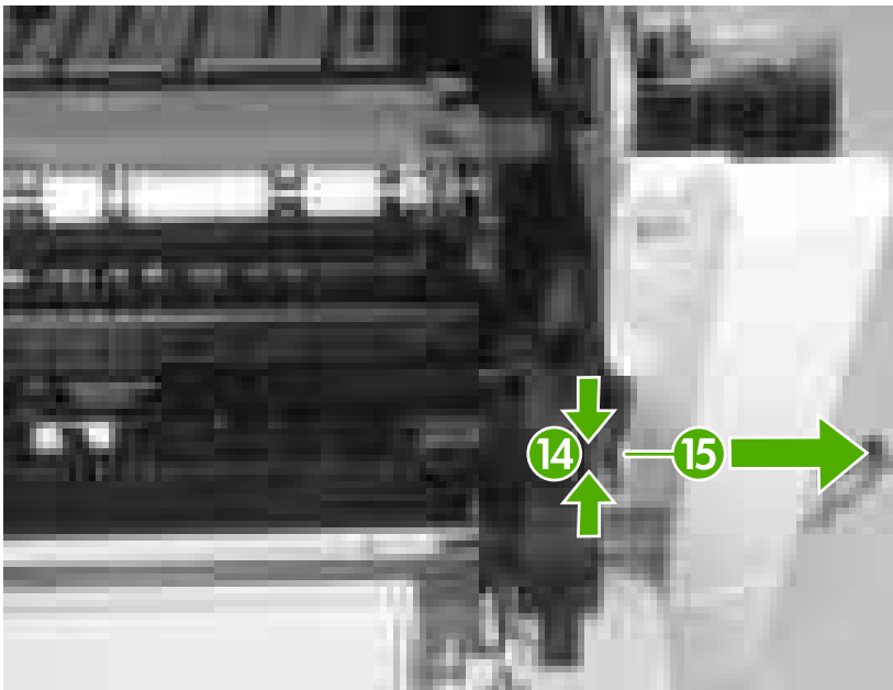
Figure 5-71 Removing the cartridge door unit (8 of 14)
