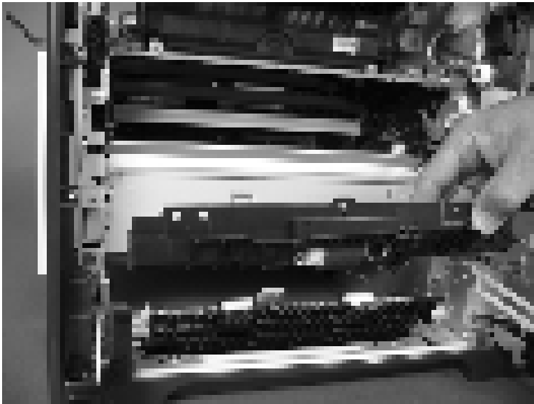
Figure 6-230 Remove the cassette-pickup assembly (3 of 3)
