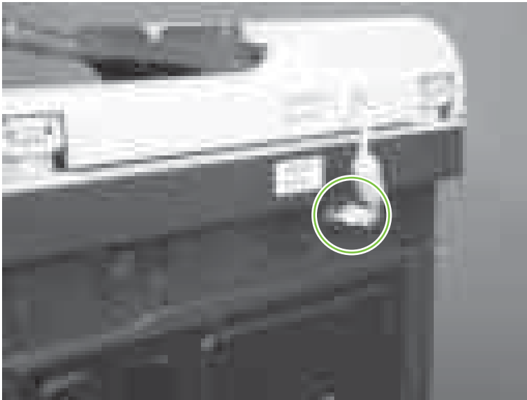
Figure 6-85 Remove the rear-upper cover (1 of 4)
