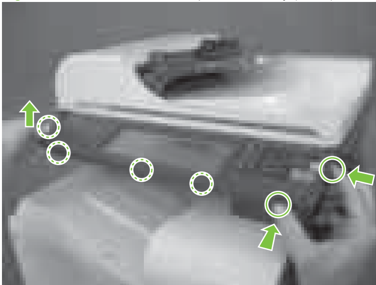
Figure 6-58 Remove the control-panel assembly (1 of 3)
