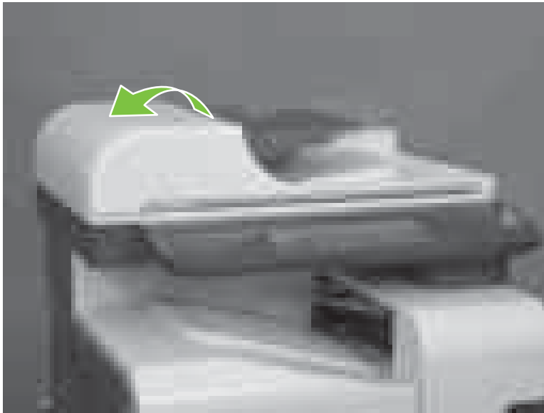
Figure 6-50 Remove the ADF roller assembly and separation pad (1 of 5)
