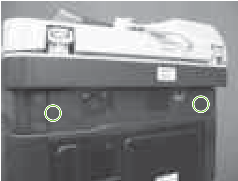
Figure 6-86 Remove the rear-upper cover (2 of 4)
